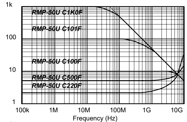
Impedance (ohm)
